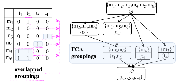
Fig. 2. A toy program and its mutant clusters
